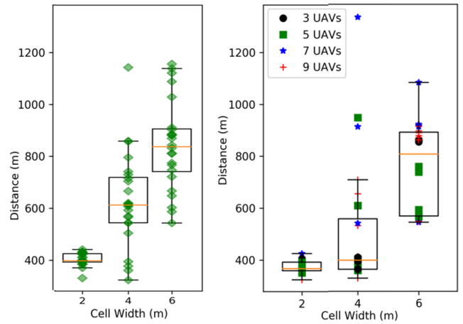
(a) Results for Peach mobility model. (b) Results for 3DGPeach mobility model. The 72 UAVs reached the model. 3 UAVs out of 72 did not reach the target.
