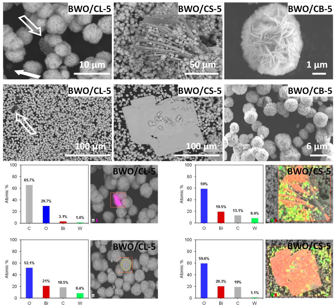
Figure 2. Selected SEM images of samples BWO/CL-5, BWO/CS-5, BWO/CB-5, arrows indicate the presence of a new phase. The EDX spectra from different regions marked with a square.
