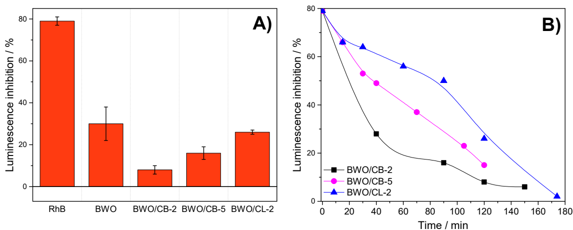
Figure 6. (A) Luminescence inhibition of BWO, BWO/CB-2, BWO/CB-5, and BWO/CL-2 photocatalysts after 120 min of irradiation, and response of the initial concentration of RhB (10 ppm) in solution; (B) Effect of the photocatalytic degradation using different BWO/carbon catalysts on the evolution of the bacteria luminescence inhibition with the irradiation time of aqueous solutions after an exposure time of 15 min.
