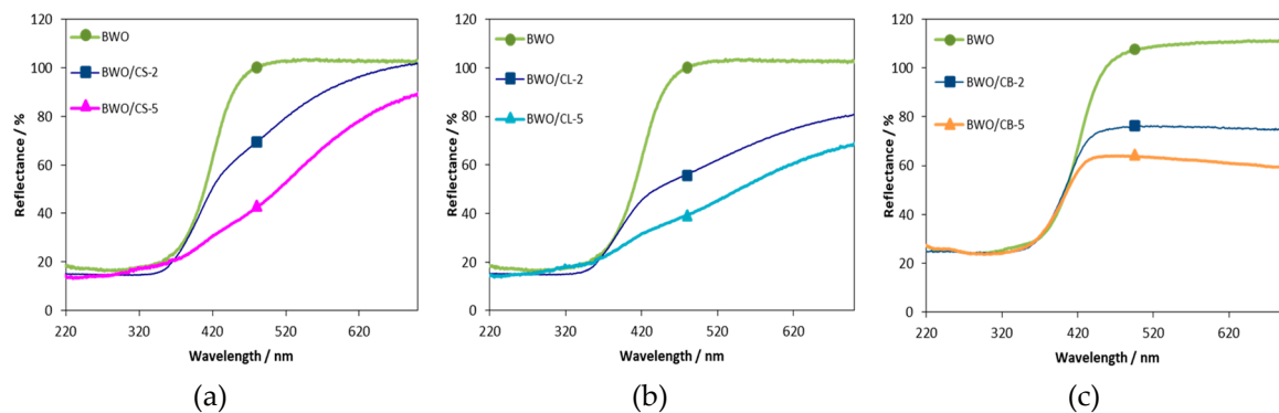
Figure 3. Diffuse reflectance spectra of Bi 2 WO 6 and the photocatalysts incorporating various amounts of the (a) CS, (b) CL and (c) CB carbon additive.
