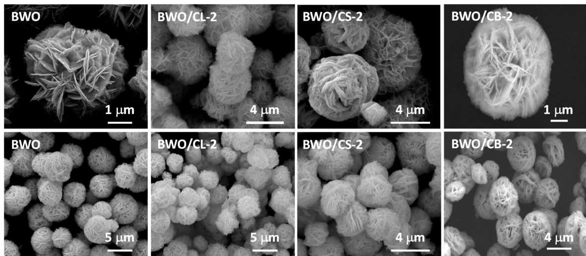
Figure 1. SEM images of Bi 2 WO 6 (BWO) and the hybrid photocatalysts containing 2 wt.% of carbon additive.
