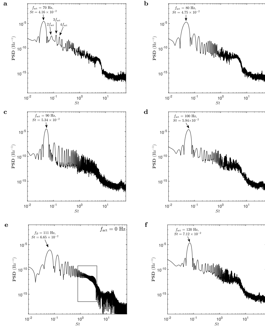
Figure 5: Power Spectral Density of the lift coefficient for different actuation frequencies, for the following frequencies: f_{\text{act}} = \{0;70;80;90;100;120\} Hz. f_{\text{act}} (fig. 5e) corresponds to the static case.
