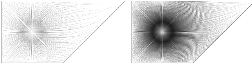
Figure 8: Trajectories of particles along the heat flow (see Rem. 5.8). Left: h = \frac{1}{30} , Right: h = \frac{1}{80} .
