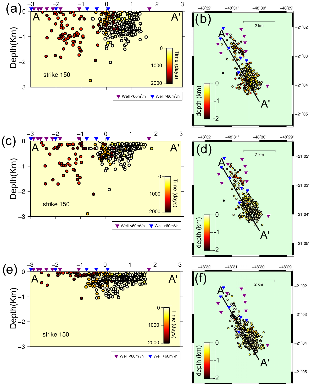
Figure 10. Hypocentral distribution of ~1000 best events (those with eight or more picks, an azimuthal gap of <math><180</math> and rms <math><0.05\text{ s}</math>) based on the use of different models. (a) and (b) Initial model 'mod0', (c) and (d) model 'mod1' and (e) and (f) final model 'mod2'. In all of the right-hand panels (b), (d) and (f), the black line A-A' in the map indicates the profile shown on the left.
