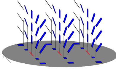
Figure 3: Visualization of the lifting: the heterogeneous tangent spaces T_{p_0}(p) defined by the multiplicity of operators are lifted to tangent planes \tilde{T}_{p_0}(p) which have all the same dimension, in a higher dimensional structure. The 2D projections of the lifted tangent planes \tilde{T}_{p_0}(p) provide the heterogeneous ones T_{p_0}(p) .
