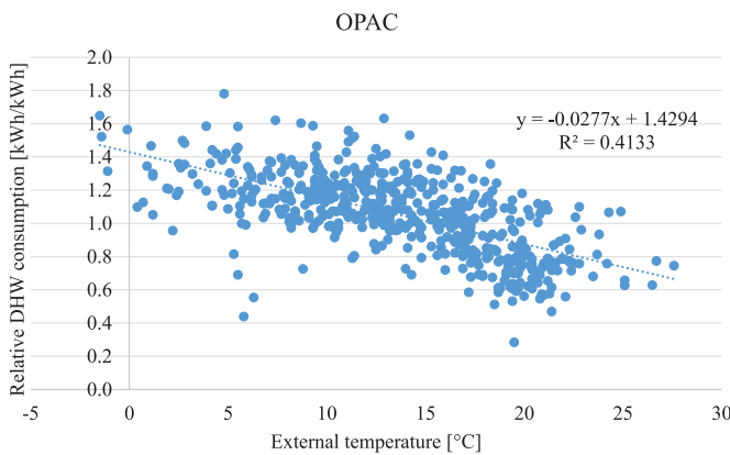
Fig. A9. Daily DHW heat consumptions of the average home in OPAC area in function of external temperature.
