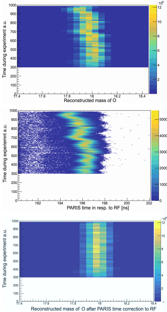
Fig. 5. Upper panel: reconstructed ^{18}\text{O} mass drift during the experimental time. Middle panel: PARIS detectors time-signal with respect to the RF, with the same drift pattern. Bottom panel: reconstructed ^{18}\text{O} mass with the RF drift corrected by using the PARIS timing information.
