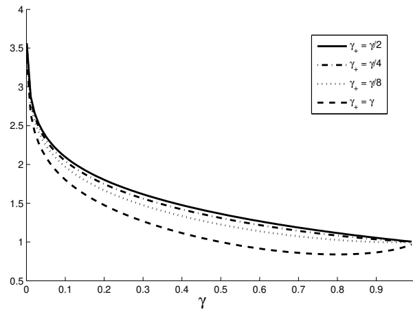
Figure 1. Function \sqrt{z_{\gamma+} \varphi(z_{\gamma+})/\gamma - z_{1-\gamma-} \varphi(z_{1-\gamma-})/\gamma + 1} as a function of the percentage \gamma of individuals genotyped, for different values of the ratio \gamma_+/\gamma .
