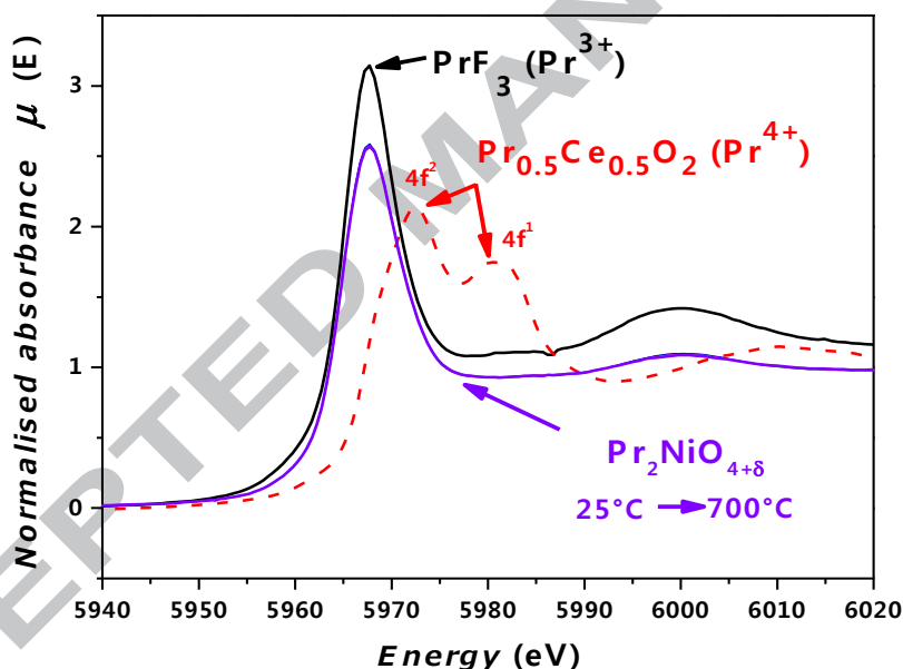
Figure 2. XANES data collected at the LIII-edge of praseodymium, for \text{PrF}_3 and \text{Pr}_{0.5}\text{Ce}_{0.5}\text{O}_2 at room temperature in air. For \text{Pr}_2\text{NiO}_{4+\delta} , the spectra were collected in the temperature range 25 - 700^\circ\text{C} in 20% \text{O}_2 diluted in helium.
