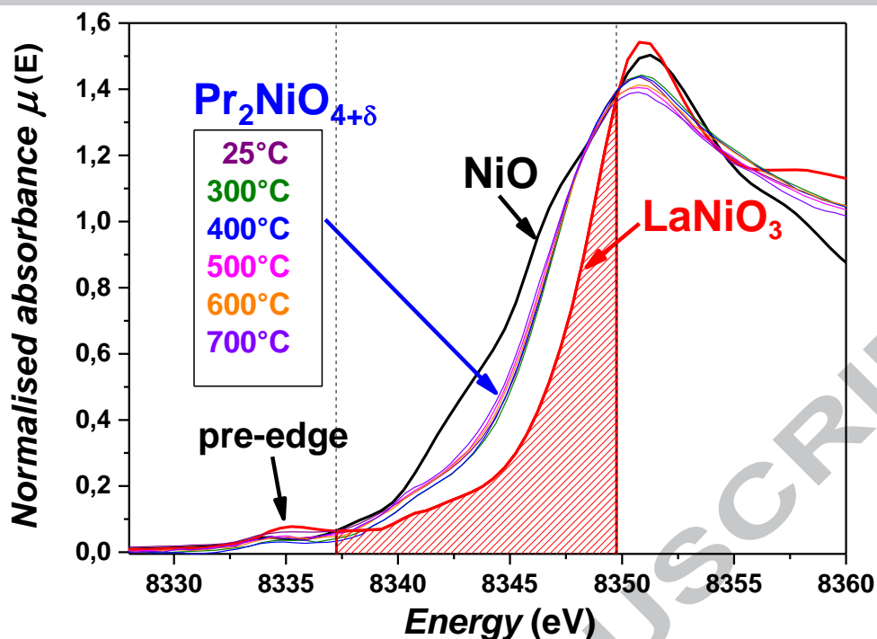
Figure 3. XANES data collected at the Ni K-edge for \text{Pr}_2\text{NiO}_{4+\delta} , in air as a function of temperature. Reference spectra of NiO and \text{LaNiO}_3 (recorded at room temperature) are given. The integration area used for \text{LaNiO}_3 (in red) is shown as an example. The pre-edge signals are indicated by an arrow.
