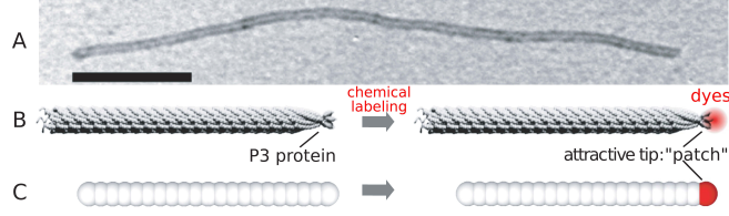
FIG. 1. (A) Transmission electron microscopy of the filamentous virus used in this work (Scale bar: 200 nm), and (B) schematic representation of pristine (left) and single-tip functionalized viral rod with red dyes (right), resulting in a localized directional attractive interaction. (C) Schematic of the semi-flexible rod-like particles, modeled as a bead-spring chain, used in computer simulations. The white beads from different particles interact via a repulsive soft-core potential, while the red ones located at one end of the rods are attractive.
