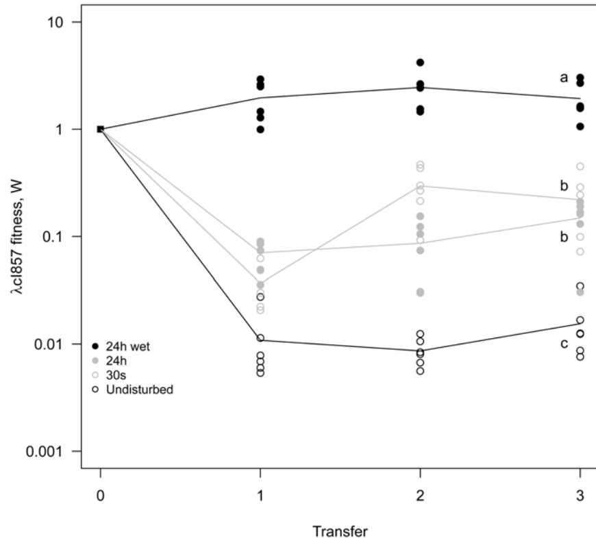
Fig 5. Mixing selects for virulence. A 1:1 mixture of temperate \lambda and its virulent mutant \lambda clI857 was used to seed spatial epidemics. Spatial structure was disturbed to different degree ( undisturbed, 30s, 24h, 24h-wet ) and transferred onto a fresh biofilm of susceptible hosts for 3 consecutive days. Disturbance of the epidemic structure has a strong effect on the competitive fitness of the virulent \lambda clI857. The undisturbed environment strongly selects against virulence whereas in a well-mixed environment ( 24h-wet ) virulence is beneficial. As expected, intermediate levels of mixing ( 30s, 24h ) lead to intermediate fitness of \lambda clI857. Symbols represent 6 replications for each mixing treatment (with 3 independent replicates for each marker-mutant combination).
