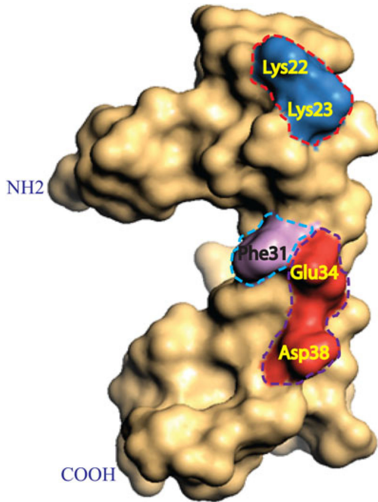
FIGURE 6. Hydrophilic residues located on the major \alpha -helix domain play important roles in release of agnoprotein. Three-dimensional structure of the full-length agnoprotein is illustrated in a “surface fill-in” representation. The hydrophilic residues located on the hydrophilic face of the major \alpha -helix domain of agnoprotein, including Lys22, Lys23, Glu34, and Asp38; and an aromatic residue (Phe31), which is adjacent to this hydrophilic surface were determined to be critical for the release of agnoprotein from agnoprotein-positive cells (Saribas, White, et al., 2018). Amino acid residues involved in agnoprotein release are encased in boxes and named. Note that Lys23, Lys23, Phe31, and Glu34 are all conserved between JCV, BKV, and SV40 agnoproteins. JCV Asp38 is substituted for Glu and Gln for BKV and SV40 agnoproteins, respectively, at the same position (Saribas, White, et al., 2018). BKV: BK virus; JCV: JC virus; SV40: simian virus 40 [Color figure can be viewed at wileyonlinelibrary.com ]
