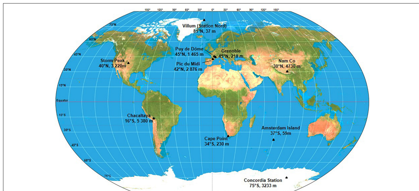
FIGURE 2 | Global distribution of the sampling sites and their respective elevation above sea level.
