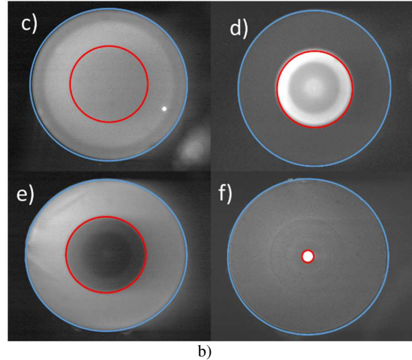
Figure 2. a) Illustration of the X-ray RIA dose dependence measured at 1550 nm at RT for four different fibers: pure-silica core (PSC), Ge-, P- and Al-doped cores b) Cathodoluminescence panchromatic images of the fiber cross sections under \sim 20 keV electron beam: c) PSC fiber with luminescence bands peaking at 450 nm, 540 nm and 650 nm from defects present in both its core (red circle) and cladding (blue circle); d) Ge-doped MMF with defects emitting around 400 nm located in its core e) P-doped MMF without luminescence in its core; f) Al-doped SMF fiber with a strong core luminescence around 350 nm. The last three fibers present the same emitting centers in their claddings than the PSC fiber.
