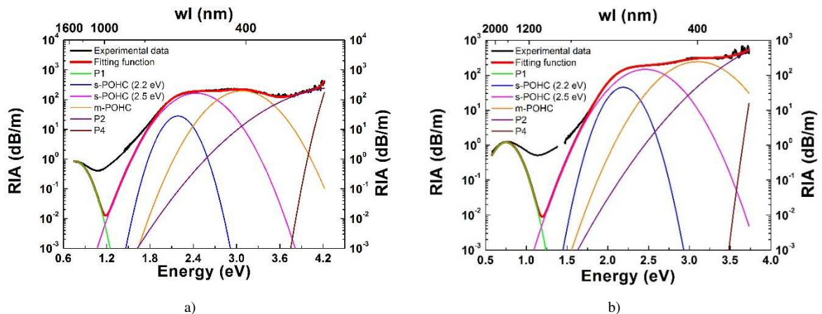
Figure 6. Illustration of the RIA spectra measured in a P-doped MMF a) 10s after an X-ray pulse at room temperature (RT, 200 Gy, > 1MGy/s) b) during X-ray irradiation at 200 Gy (RT) at 100 mGy/s. The best achievable fits are reported using the set of defects described in Table 3 and the corresponding OA bands.
