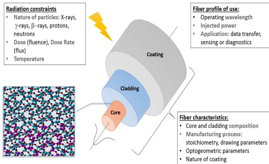
Figure 1. Main parameters affecting the radiation response of a silica-based optical fiber in terms of RIA, RIE and RIRIC. The fiber structure is illustrated as well as the nature of the glass at the core and cladding interface. The inset illustrates a typical silica model used for ab initio calculation of the point defect properties: core is made of Ge-doped silica and the cladding is in pure silica (Si atoms are in red, Oxygen ones in green and Ge atoms in purple).
