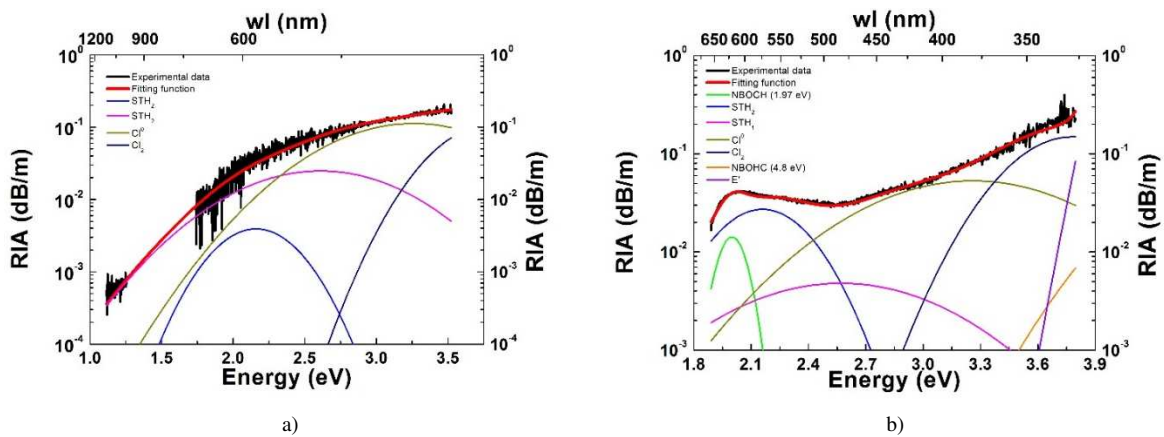
Figure 4. Illustration of the RIA spectra measured in a PSC solarization resistant multimode optical fiber (MMF) a) 1 s after an X-ray pulse at RT b) during \gamma -ray irradiation at 200 Gy (RT) with a dose rate of 3 mGy/s. The best achievable fits are reported using the set of defects described in Table 1 and the OA bands of the defects involved in the fiber response.
