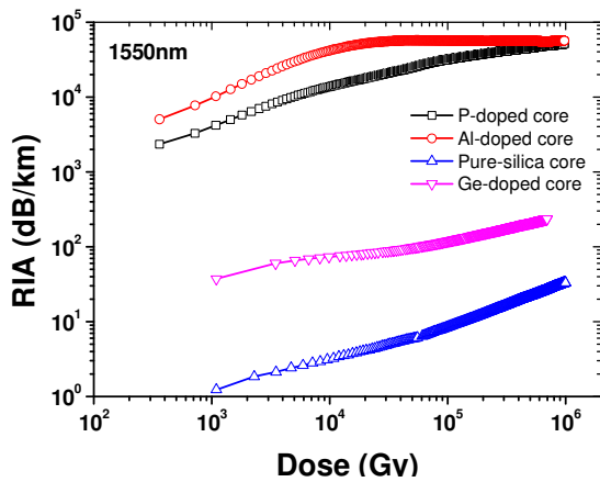
Figure 2. a) Illustration of the X-ray RIA dose dependence measured at 1550 nm at RT for four different fibers: pure-silica core (PSC), Ge-, P- and Al-doped cores b) Cathodoluminescence panchromatic images of the fiber cross sections under \sim 20 keV electron beam: c) PSC fiber with luminescence bands peaking at 450 nm, 540 nm and 650 nm from defects present in both its core (red circle) and cladding (blue circle); d) Ge-doped MMF with defects emitting around 400 nm located in its core e) P-doped MMF without luminescence in its core; f) Al-doped SMF fiber with a strong core luminescence around 350 nm. The last three fibers present the same emitting centers in their claddings than the PSC fiber.
