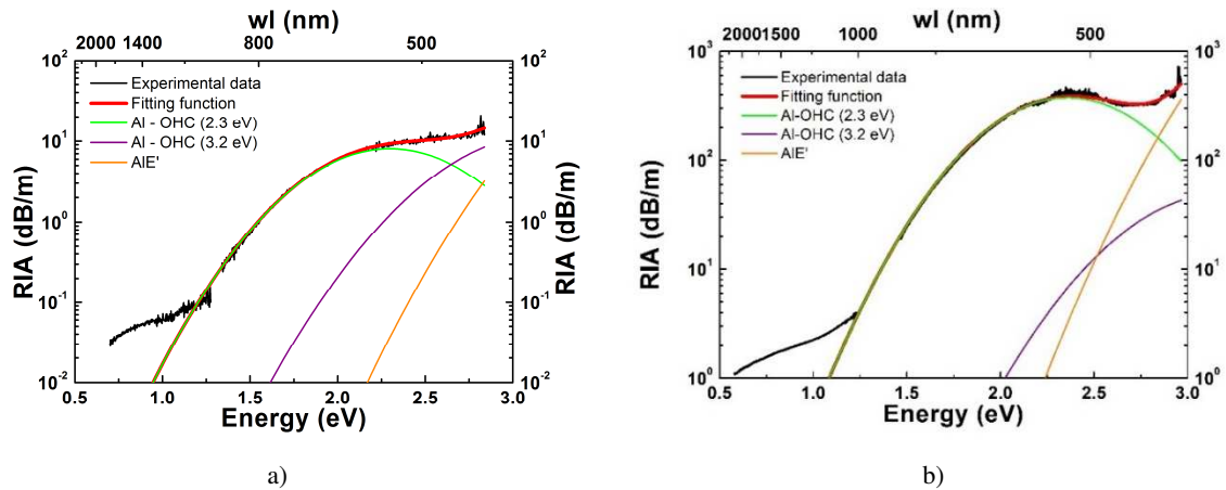
Figure 7. Illustration of the RIA spectra measured in an Al-doped MMF a) 1 s after a pulsed X-ray (6.2 Gy, > 1MGy/s) b) during X-ray irradiation at 200 Gy (RT) at 100 mGy/s. The best achievable fits are reported using the set of defects described in Table 4 and the contributing OA bands.
