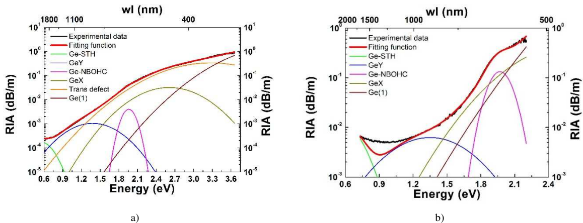
Figure 5. Illustration of the RIA spectra measured in a Ge-doped MMF a) 1s after an X-ray pulse at room temperature (RT, 200 Gy, > 1MGy/s) b) during γ-ray irradiation at 200 Gy (RT) at 4 mGy/s. The best achievable fits are reported using the set of defects described in Table 2 and the corresponding OA bands.
