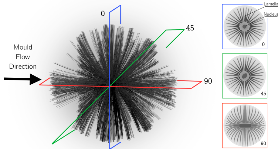
Figure 14: Oriented spherulitic structure induced by the injection molding.
