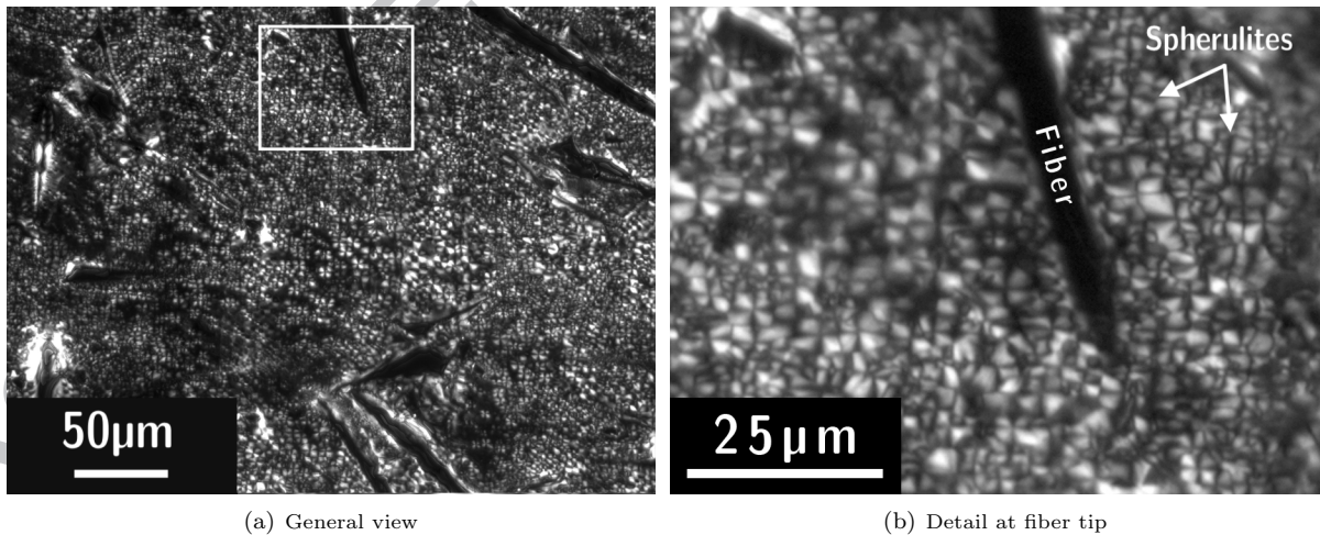
Figure 3: Spherulites observed using polarized light microscopy on thin slices of reinforced PA66 obtained by microtomy. Slicing was performed in a longitudinal direction compared to fibers, which gives better view of the microstructure but is more challenging than transversal cut as usually performed for bulk composite material [6, 13].
