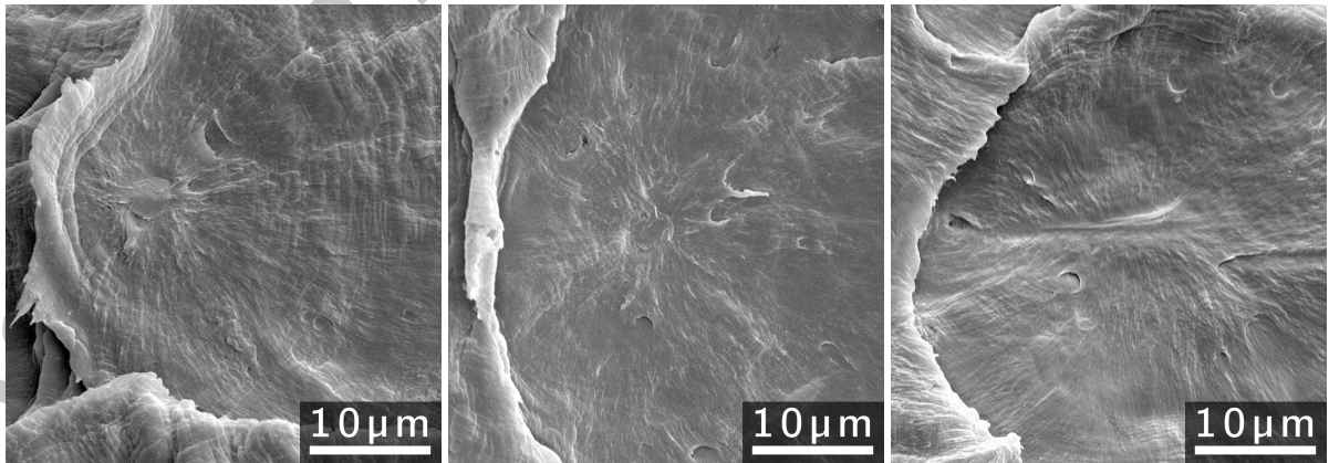
(a) 0° specimen
