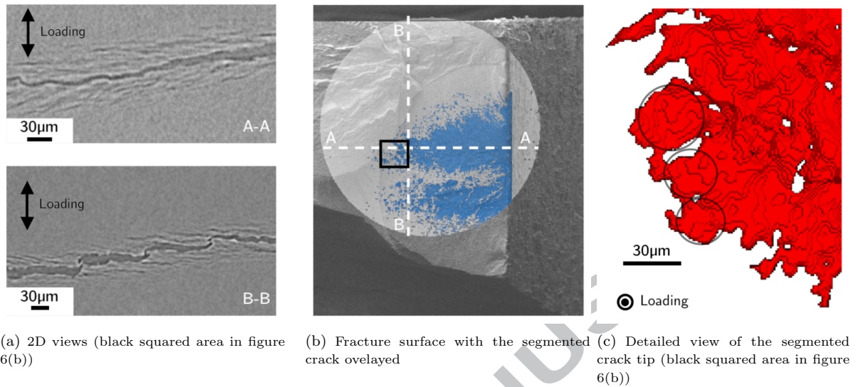
Figure 6: Crack tip in a PA66 notched specimen as observed by microtomography, test interrupted at 2531 cycles and 95% of estimated fatigue life.
