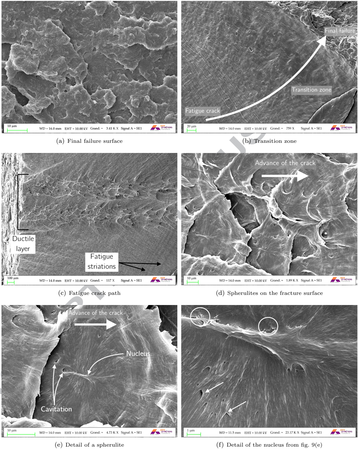
Figure 9: SEM fractography of a notched PA66 specimen ( N_f = 917 ).
