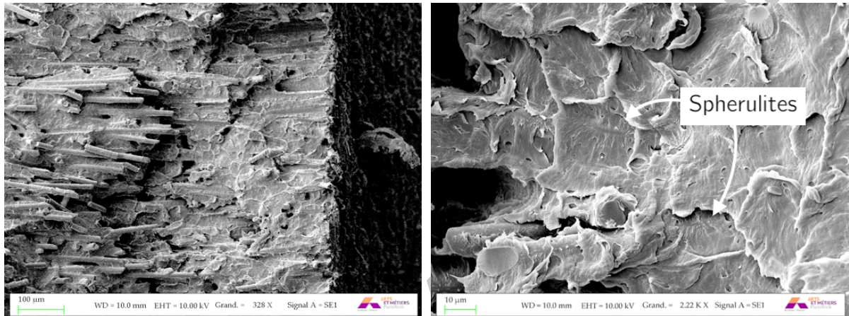
(a) Fatigue crack path in the core of the specimen
