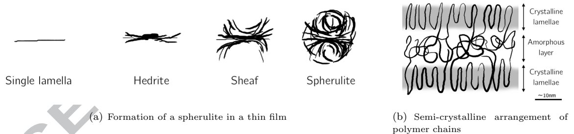
Figure 1: Formation and structure of spherulites in a semi-crystalline thermoplastic.
