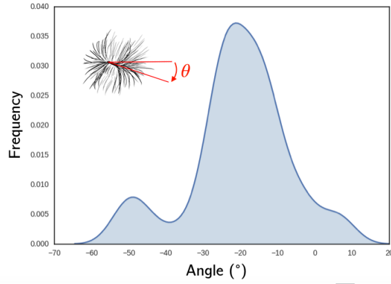
Figure 12: Orientation of the 40 nuclei observed on 3 different PA66 specimens after fatigue testing.
