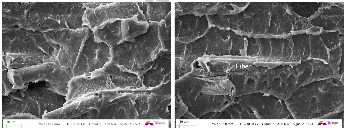
(c) Spherulites and fibers on the fracture surface
