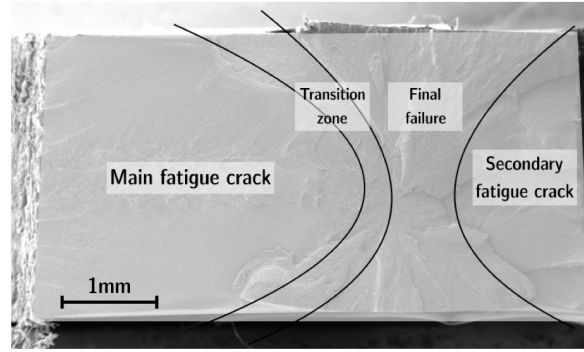
Figure 8: Fracture surface of a notched PA66 specimen after fatigue testing ( N_f = 917 ).
