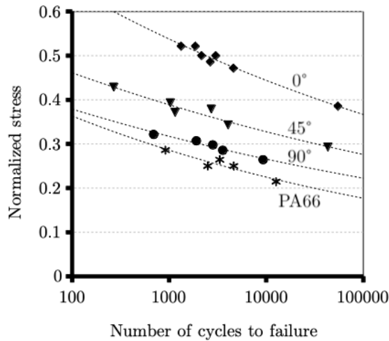
Figure 4: Geometries and S-N curves for the notched specimens.
