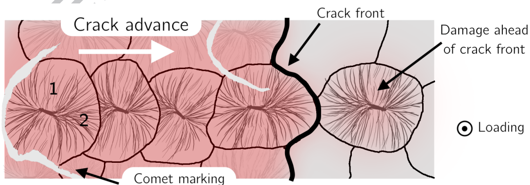
Figure 11: Schematic of the influence of the spherulitic structure of the polymer on fatigue crack advance.
