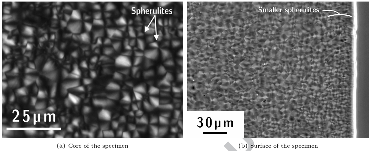
Figure 2: Spherulites in PA66 observed using polarized light microscopy on thin slices obtained by microtomy.
