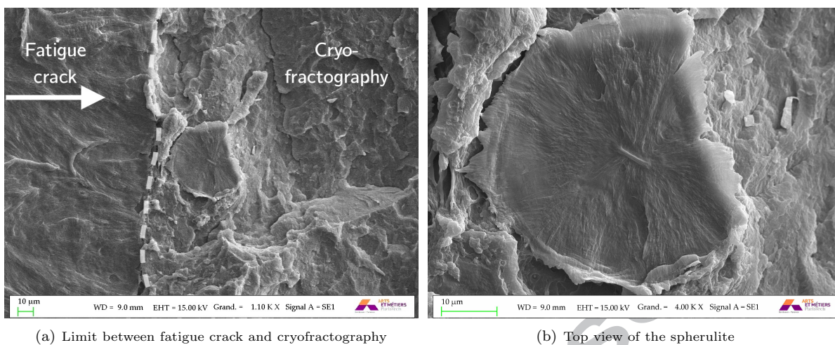
Figure 10: Spherulitic damage ahead of the fatigue crack in a notched PA66 specimen after cryofractography, test interrupted at 4221 cycles and 90% of estimated fatigue life.
