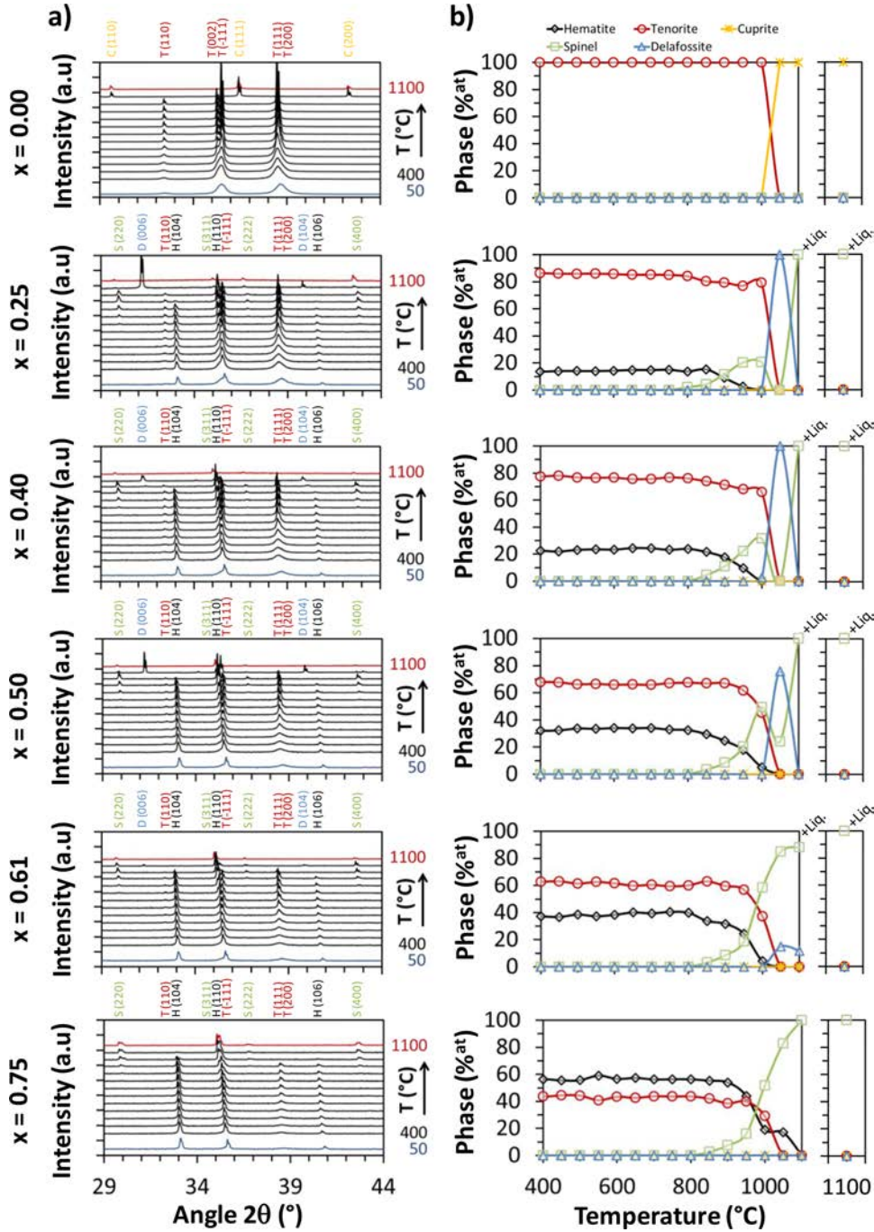
Figure 2. (a) XRD patterns for the samples x = 0.00, 0.25, 0.40, 0.50, 0.61, and 0.75 over the temperature range 50–1100 ^\circ\text{C} . (b) Corresponding amount of crystalline phases quantified by Rietveld refinement.
