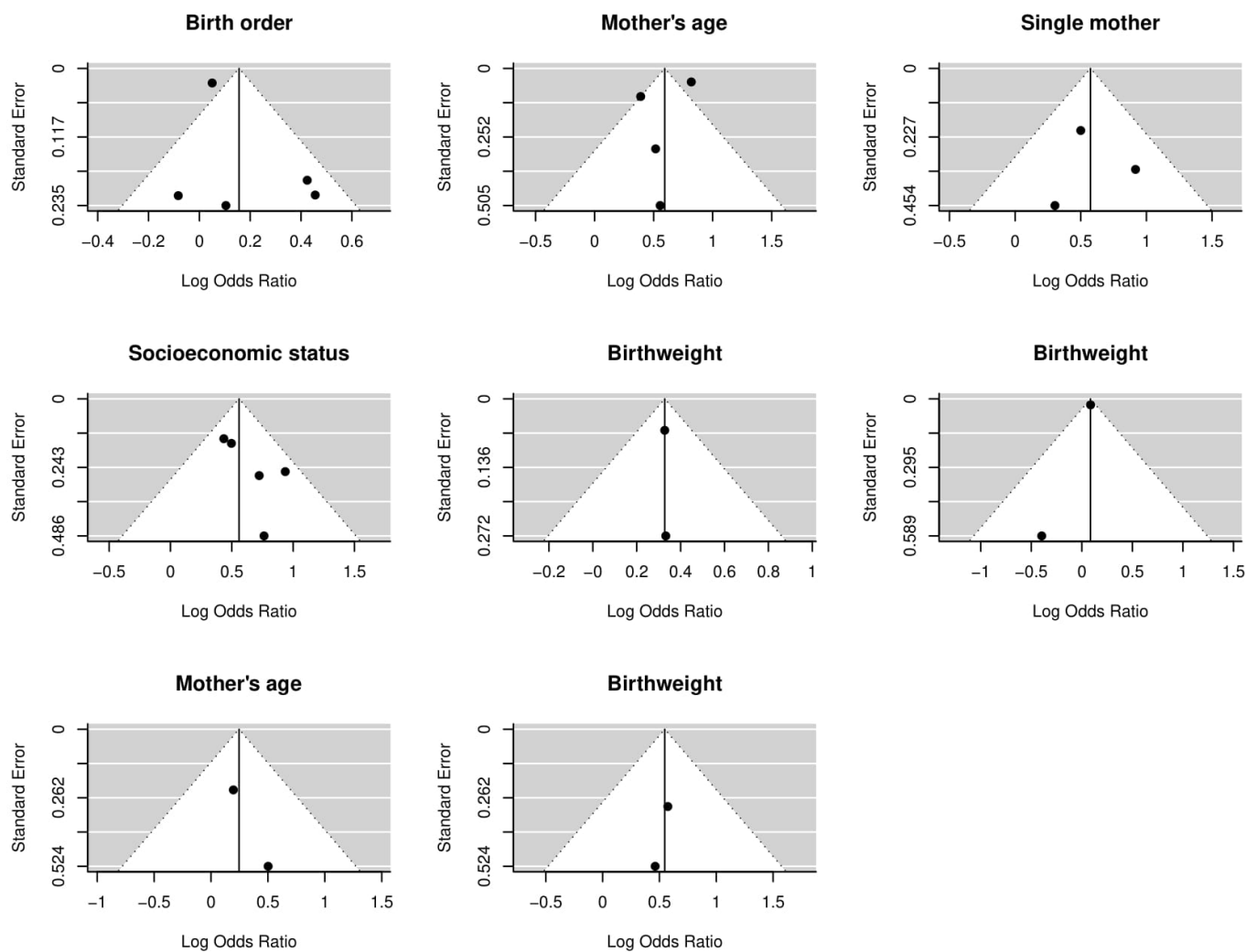
Supplementary Figure 2. Funnel plot for suicide attempt and suicidal ideation
