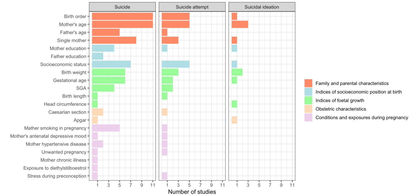
Figure 2. Assessed risk factors across the included studies
