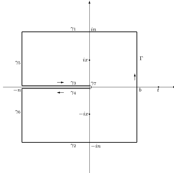
FIGURE 1. The contour of integration.
