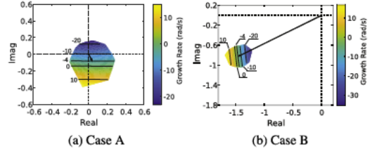
Fig. 8. Modal growth rate contours in generalized phasor plot of FRF. Black lines are the contour levels predicted by the analytical approach. For each case, Line with black arrow is the F(\omega^0) phasor evaluated by using nominal values of h_k 's, which corresponds to a growth rate value of -4 rad/s.
