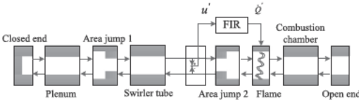
Fig. 6. Sketch of the acoustic network model. Flow from left to right.
