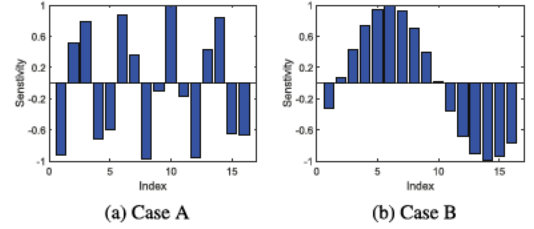
Fig. 11. Sensitivity measurements for each FIR model coefficients.
