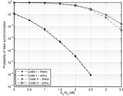
Figure 2: Hard synchronization of LDPC codes
