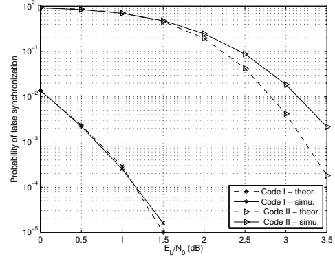
Figure 3: Soft synchronization of LDPC codes
