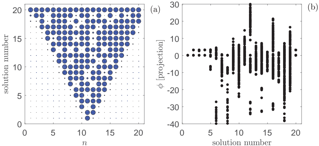
Figure 9 - (a) Localized states for \tilde{v}_d = 1.65 . Each circle represents a oscillator, with the radius proportional to the amplitude of the vibration.
