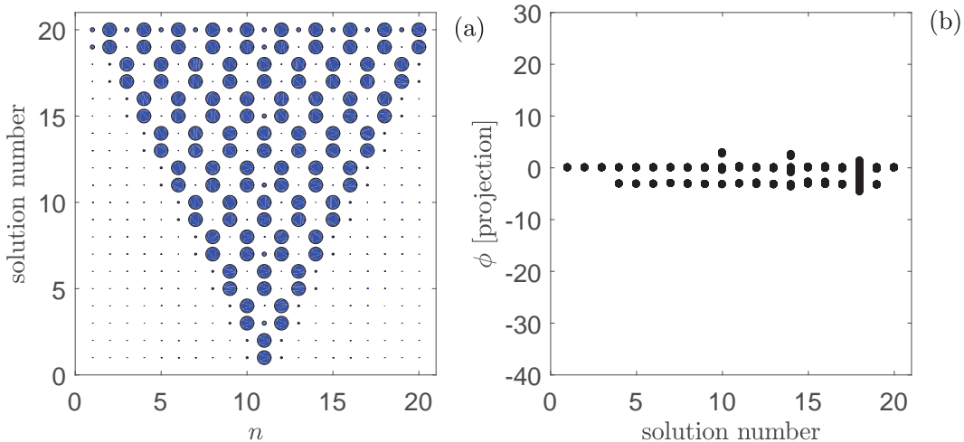
Figure 10 - (a) Localized states for \tilde{v}_d = 1.75 and \tilde{x}_n(0) > 0 ( \forall n ). Each circle represents a oscillator, with the radius proportional to the amplitude of the vibration. (b) Orbit diagram (as in Fig. 8) for the solution in the panel (a)
