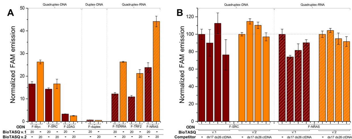
Figure 4. (A) One-step pull-down results (FAM intensity of F-ON after release from the beads) for experiments carried out with 1 \mu M of G4-DNA (F-Myc, F-SRC and F-22AG, plain bars), ds-DNA (F-duplex, cross-hatched bars) or G4-RNA (F-TERRA, F-TRF2 and F-NRAS, diagonally hatched bars) and 20 \mu M of both BioTASQ (v.1 and v.2, brown and orange bars, respectively). (B) Competitive pull-down experiments carried out with 1 \mu M of G4-DNA (F-SRC) or G4-RNA (F-NRAS), 20 \mu M of both BioTASQ (v.1 and v.2) in absence or presence of competitive ds-DNA (either 20 \mu M of ds17 or ds26, or 100 \mu M of calf thymus DNA (ctDNA)).
