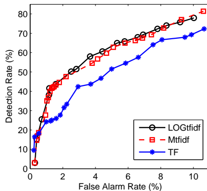
Fig. 1. ROC curves for PCA method with various different frequency weights
