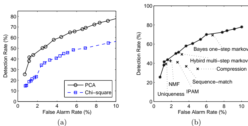
Fig. 2. (a): ROC curves for PCA and X^2 test method using LOGtfidf weight; (b): ROC curves for PCA method using LOGtfidf weight along with the results from other 7 methods
