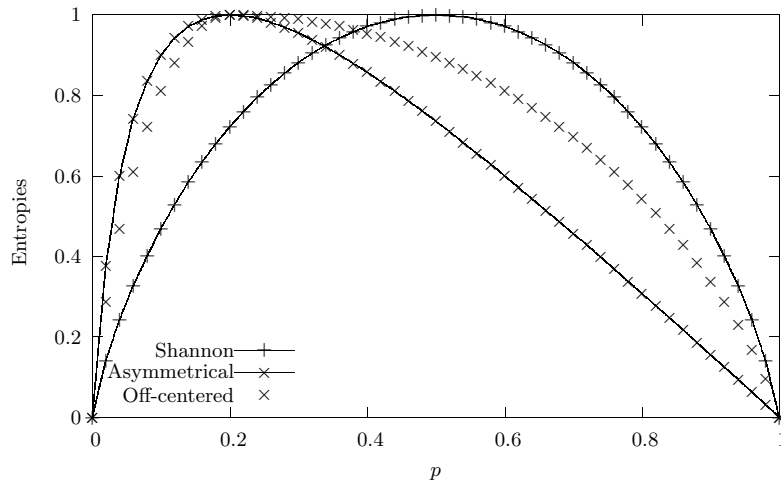
Fig. 1. Off-centered, asymmetric and Shannon's entropies
