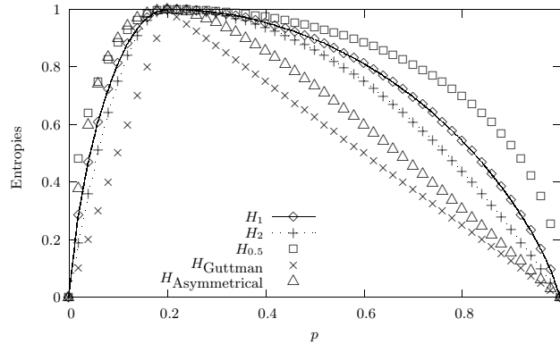
Fig. 2. Off-centering of generalised entropies
