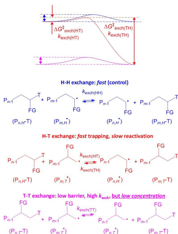
Figure 7. Mechanisms and energy profiles of the associative exchange processes involving head and tail dormant species with head and tail radicals in controlled polymerization of asymmetric monomers.
