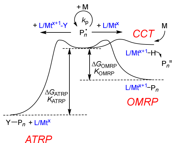
Figure 1. Interplay between ATRP, OMRP and CCT processes. All symbols are defined in the schemes and within the text.
