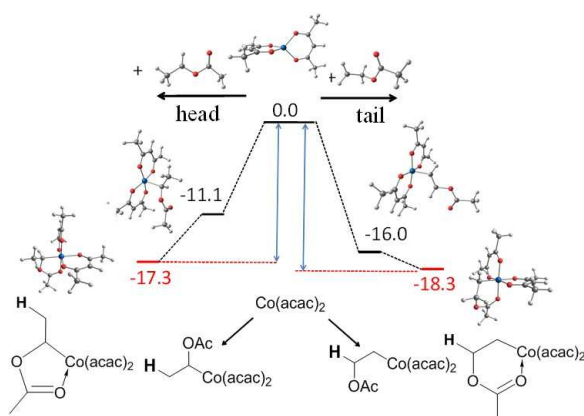
Figure 9. Energy profile (relative H values in kcal/mol) and views of the optimized geometries for the trapping of head and tail PVAc model radicals \text{CH}_3\text{CH}(\text{OAc})^\bullet and ^\bullet\text{CH}_2\text{CH}_2(\text{OAc}) [69].
