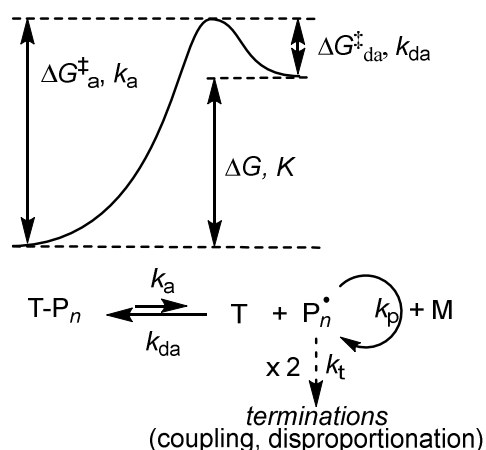
Scheme 1. Mechanism and activation/deactivation free energy profile of a controlled radical polymerization based on reversible termination. P_n = polymer chain with degree of polymerization n , T = radical trapping species, M = monomer.
