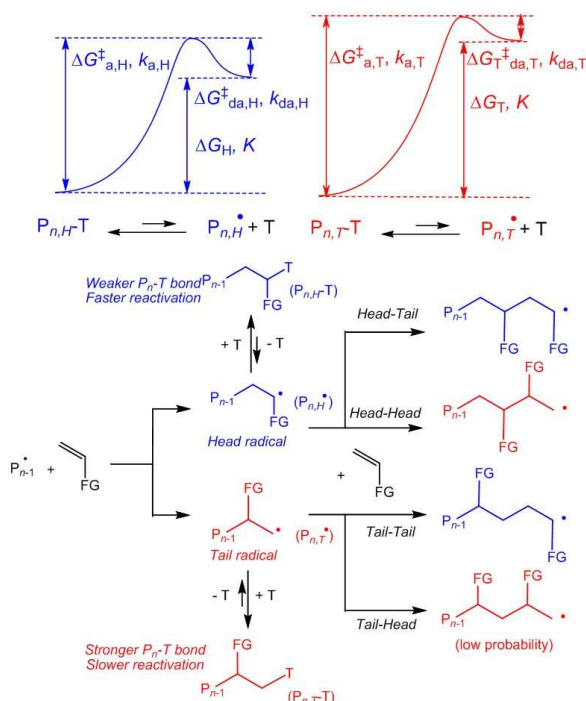
Figure 6. The problem of the inverted monomer additions for LAMs.
