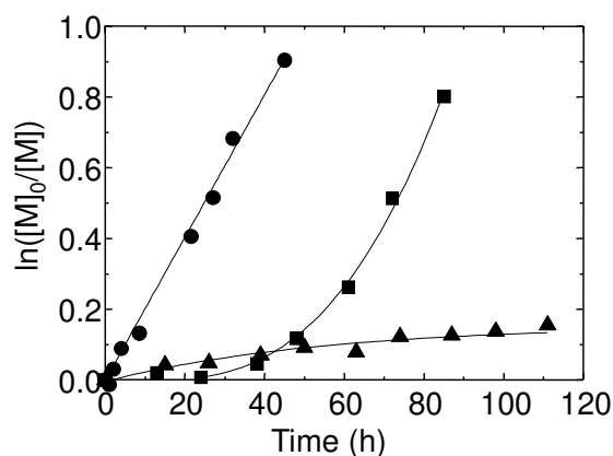
Figure 2. Effect of the addition of external ligands (L) to kinetics of the bulk OMRP of VAc mediated by [\text{Co}(\text{acac})_2] with V-70 at 30^\circ\text{C} ( [\text{VAc}]_0/[\text{Co}(\text{acac})_2]_0/[\text{V-70}]_0/[\text{L}]_0 = 500:1:1:30 ). (■) no addition, (●) addition of py (30 equiv), (▲) addition of \text{NEt}_3 (30 equiv). Reproduced with permission from ref. [45]. Copyright 2007 Wiley-VCH.
