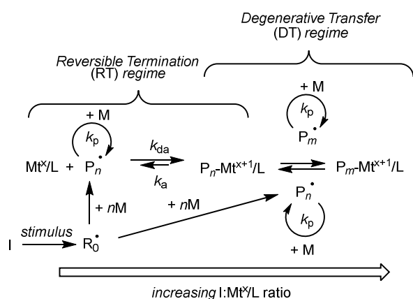
Scheme 5. Interplay of RT and DT OMRP when starting the polymerization with a dual initiating system. I = initiator, R_0 = primary radical. The other symbols have the same meaning as in Scheme 1 and Scheme 3.
