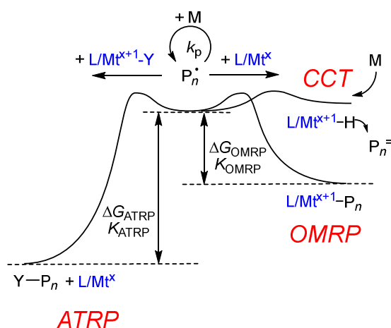
Figure 1. Interplay between ATRP, OMRP and CCT processes. All symbols are defined in the schemes and within the text.
