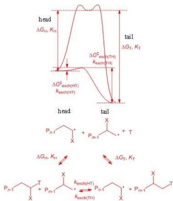
Figure 8. Thermodynamic cycle involving the non-degenerate head-tail exchange and the dissociative equilibria of the individual head and tail dormant species.
