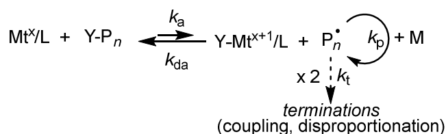
Scheme 4. Mechanism of atom transfer radical polymerization. Y = halogen atom. The other symbols have the same meaning as in Scheme 1 and Scheme 3.
