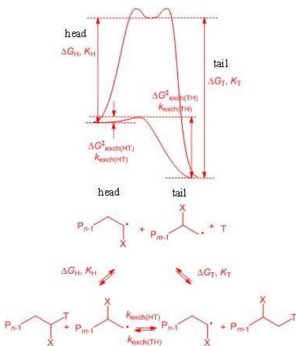
Figure 8. Thermodynamic cycle involving the non-degenerative head-tail exchange and the dissociative equilibria of the individual head and tail dormant species.
