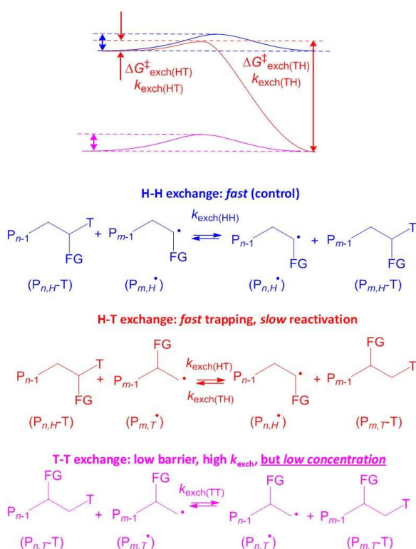
Figure 7. Mechanisms and energy profiles of the associative exchange processes involving head and tail dormant species with head and tail radicals in controlled polymerization of asymmetric monomers.
