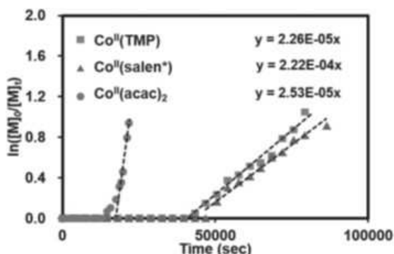
Figure 3. First order kinetic plot for the bulk VAc polymerization mediated by different cobalt(II) complexes with AIBN at 60°C ( [VAc]_0/[Co^{II}]_0/[AIBN]_0 = 700:1:3 ). Reproduced with permission from ref. [47]. Copyright 2016 Wiley-VCH.
