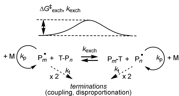
Scheme 2. Mechanism and free energy profile of a controlled radical polymerization based on degenerative transfer. The symbols have the same meaning as in Scheme 1.
