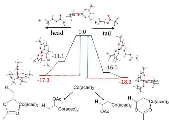
Figure 9. Energy profile (relative H values in kcal/mol) and views of the optimized geometries for the trapping of head and tail PVAc model radicals \text{CH}_3\text{CH}(\text{OAc})\cdot and \cdot\text{CH}_2\text{CH}_2(\text{OAc}) [69].
