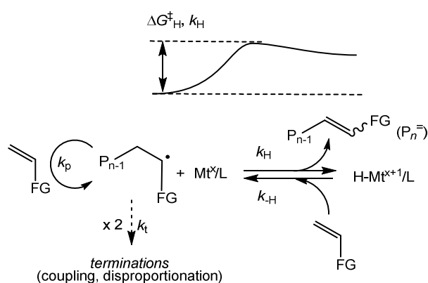
Scheme 3. Mechanism and free energy profile of metal-catalyzed chain transfer to monomer (CCT). FG stands for “functional group”. Mt = metal, x = formal oxidation state, /L = coordination sphere. P_n has the same meaning as in Scheme 1; P_0 = H .
