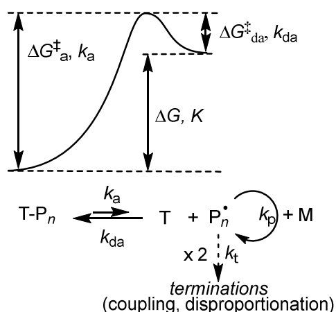
Scheme 1. Mechanism and activation/deactivation free energy profile of a controlled radical polymerization based on reversible termination. P_n = polymer chain with degree of polymerization n , T = radical trapping species, M = monomer.
