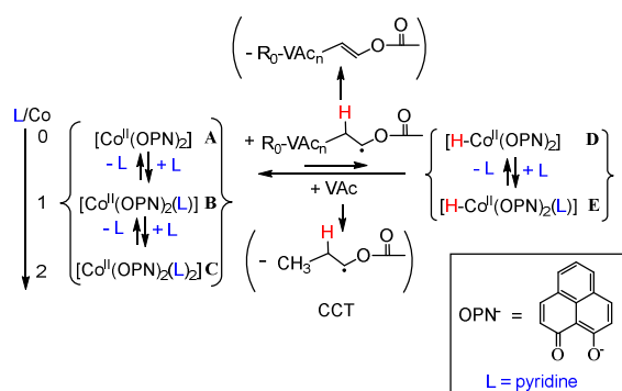
Scheme 7. Mechanism of [\text{Co}^{\text{II}}(\text{OPN})_2] -catalyzed chain transfer (CCT) in VAc polymerization and effect of L coordination.
