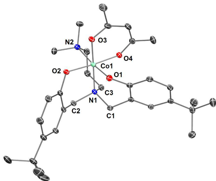
Figure 5. View of the molecular structure of 6 . The hydrogen atoms are omitted for clarity. Ellipsoids are represented at the 30% probability level. Selected bond lengths (Å) and angles (deg) are given in Table 1.
