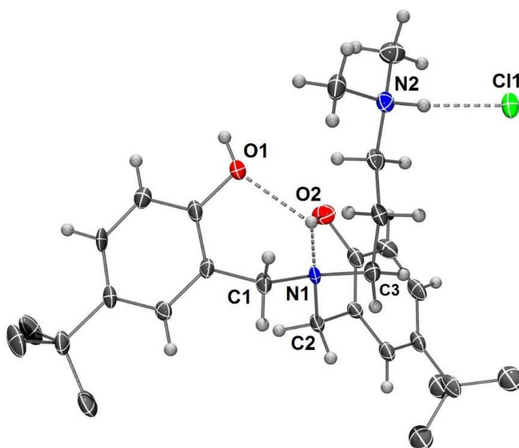
Figure 1. View of the molecular structure of \mathbf{2} \cdot \text{H}_3\text{Cl} . Hydrogen atoms of the \text{tBu} groups omitted for clarity. Ellipsoids are represented at the 30% probability level. Selected bond lengths ( \text{\AA} ) and angles (deg): N1-C1 1.478(6), N1-C2 1.478(6), N1-C3 1.493(6), N1-O2 2.671(6), N2-Cl1 3.039(5), C1-N1-C2 109.9(4), C1-N1-C3 111.1(4), C2-N1-C3 109.2(4).
