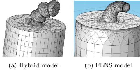
Figure 6: Examples of meshes used in the hybrid model and FLNS model
