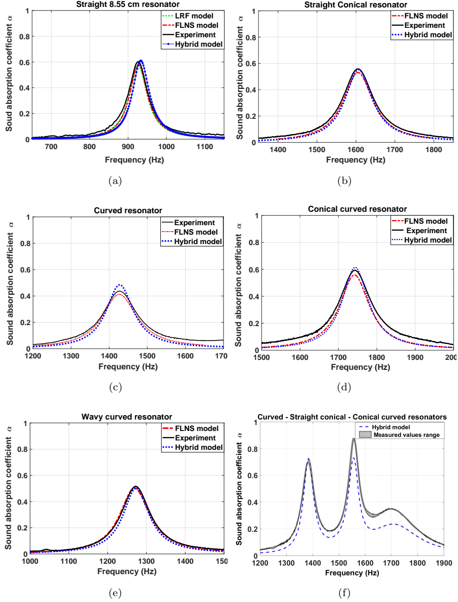
Figure 10: Sound absorption coefficient of the six quarter-wave resonator based absorbers presented above (Cf. Fig.5 and Fig.7)
