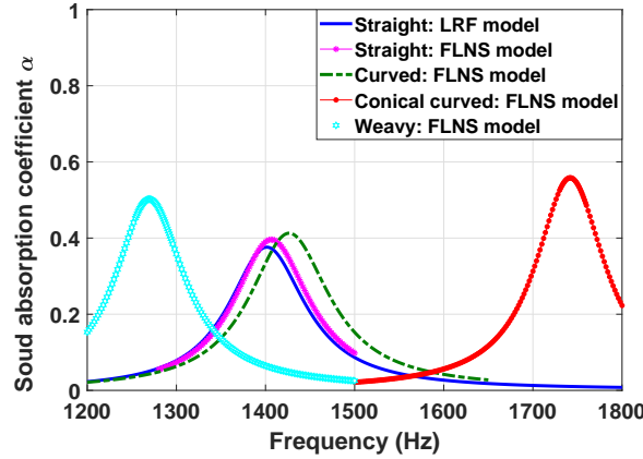
Figure 11: Sound absorption of different quarter-wave based resonators having the same the central curvilinear length of 5.526cm at the same temperature (31.5°C). The curves of this figure show the effect of resonator geometry for a given length.
