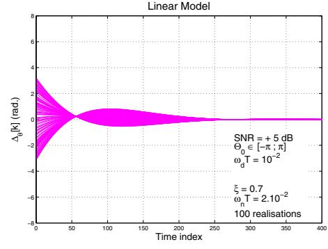
Fig. 4. Phase error signal \Delta_{\theta}[k] , SNR = +5 \text{ dB} , \omega_d T = 0.01 .
