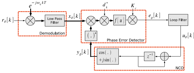
Fig. 1. Block diagram of a digital data-aided carrier demodulator
