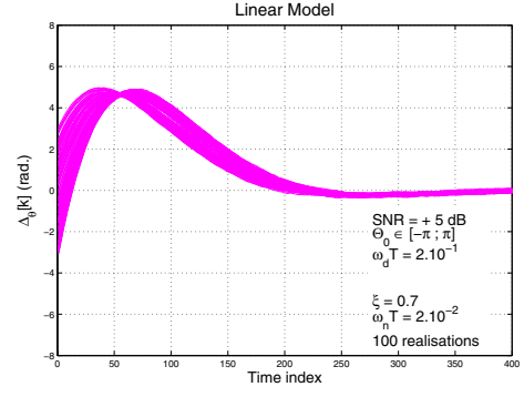
Fig. 9. Phase error signal \Delta_\theta[k] , SNR = +\infty , \omega_d T = 0.2 .
