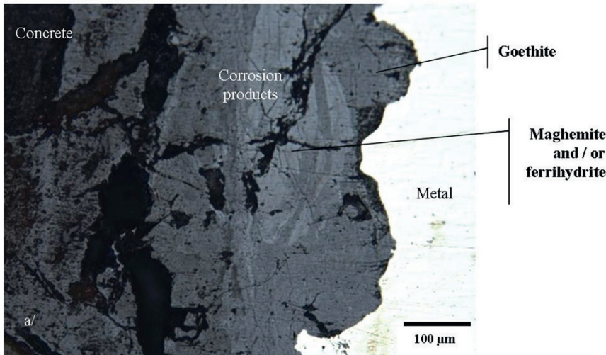
Figure 5: Microphotography (a) and Raman spectra (b and c) of a corrosion layer of the third type, 532 nm, 80 \mu W, 300s acquisition
