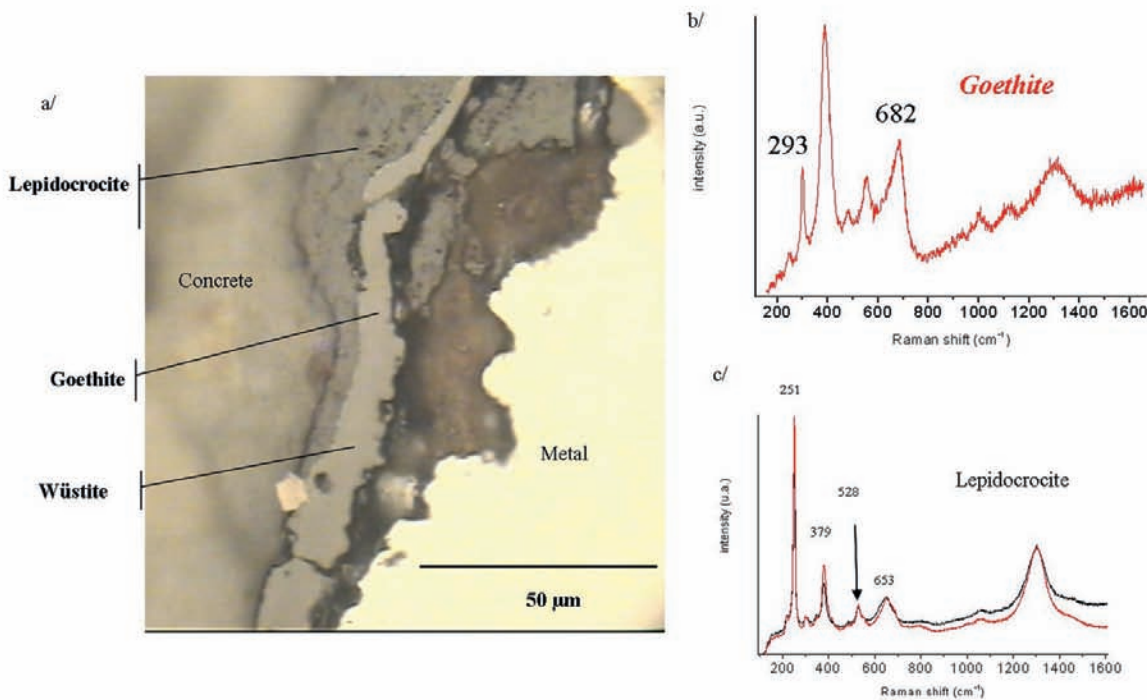
Figure 4: Microphotography (a) and Raman spectra (b and c) of a corrosion layer of the second type, 532 nm, 80 \mu W, 300 s acquisition, ONERA sample
