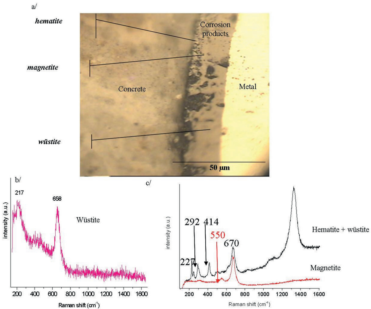
Figure 3: Microphotography (a) and Raman spectra (b and c) of a corrosion layer of the first type, 532 nm, 80 µW, 300s acquisition, “Bourse du Travail” sample
