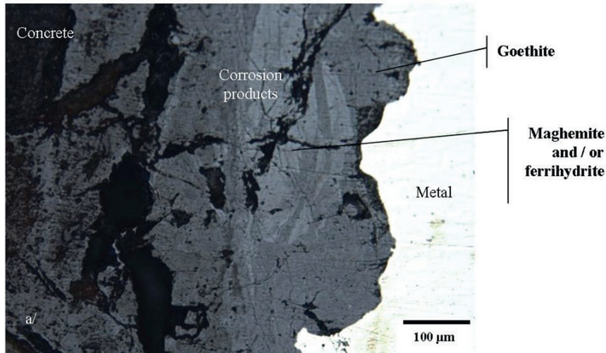
Figure 5: Microphotography (a) and Raman spectra (b and c) of a corrosion layer of the third type, 532 nm, 80 μW, 300s acquisition
