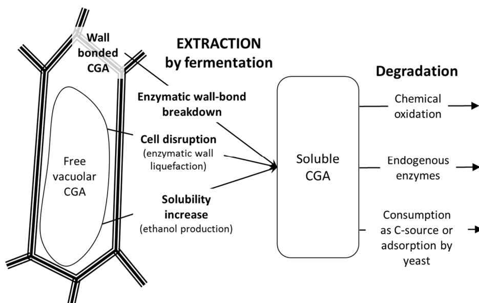
370 Fig. 3. Suggested competing pathways of the extraction and degradation of chlorogenic acids 371 (CGA) during fermentation of coffee pulp.
