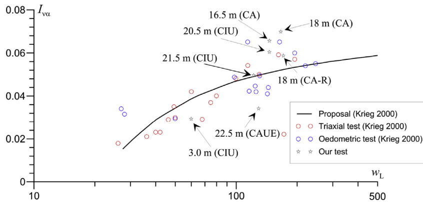
Fig. 16. Experimental observation of viscosity index (Krieg, 2000).
