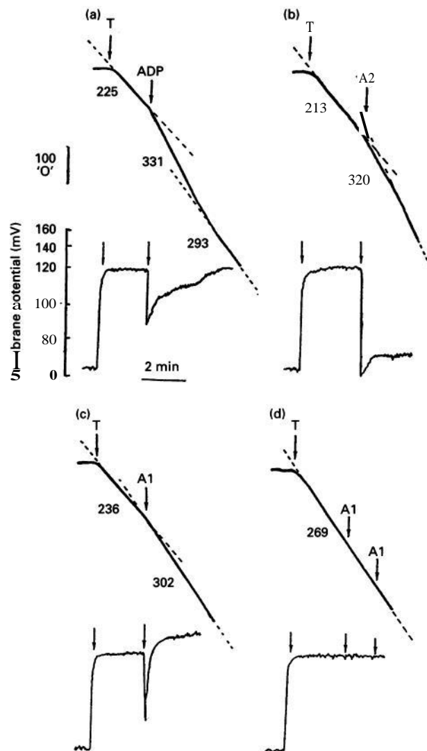
Figure 5 Effect of ADP and ATP on oxygen consumption (upper thick traces) and membrane potential (lower thin traces) of yeast mitochondria oxidizing TMPD/ascorbate
