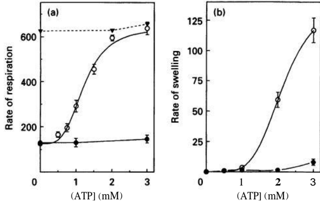
Figure 1 Effect of increasing ATP concentrations on the rate of respiration (a) and swelling in potassium acetate (b) of S. cerevisiae mitochondria
