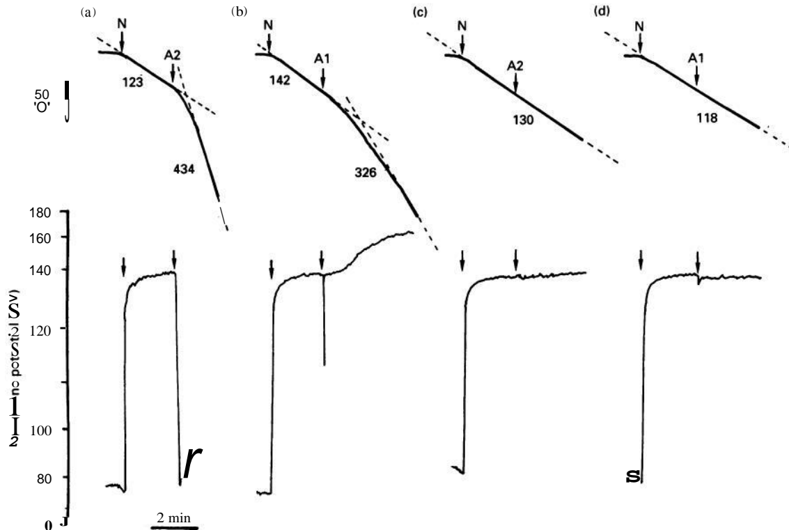
Figure 2 Effect of ATP on oxygen consumption (upper thick traces) and membrane potential (lower thin traces) of yeast mitochondria oxidizing NADH
