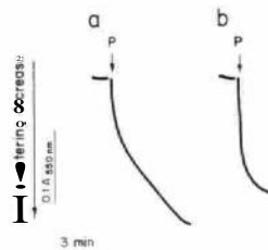
Fig. 1. Effect of 4 nmol/mg CA(1-8)M(1-18)-NH 2 on the permeability to sucrose (a) and potassium acetate (b) of rat liver mitochondria. Permeabilities were determined from the rate of light-scattering decrease during osmotic swelling when mitochondria were suspended either in 250 mM sucrose or 100 mM potassium acetate. See Materials and Methods for further details. Peptide was added when indicated. P.
