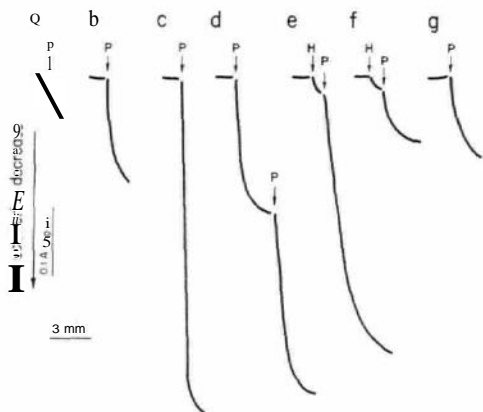
Fig. 2. Effect of varying concentrations of CA(1-8)M(1-18)-NH 2 and heparin on the swelling of mitochondria in potassium acetate. (a) 2 nmol peptide/mg mitochondrial protein; (b) 4 nmol/mg; (c) 8 nmol/mg; (d) two consecutive additions of 4 nmol/mg; (e), heparin 0.13 mg/ml plus 4 nmol peptide/mg mitochondrial protein; (f) heparin 0.65 mg/ml plus 4 nmol peptide/mg; (g) addition of a previously incubated mixture of 4 nmol peptide/mg plus 0.13 mg heparin/ml. Additions: H, heparin; P, peptide CA(1-8)M(1-18)-NH 2 .
