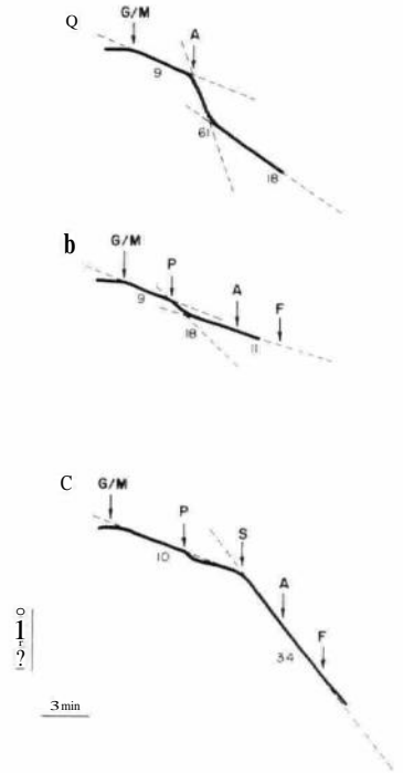
Fig. 4. Effect of CA(1-8)M(1-18)-NH 2 on mitochondria respiring with glutamate and malate as substrate. (a) Control mitochondria; (b) effect of 3 nmol peptide/mg; (c) effect of 5 nmol/mg. Additions: G/M, 5 mM glutamate plus 5 mM malate; A, 0.2 mM ADP; S, 5 mM succinate; F, 10 pM FCCP; P, peptide CA(1-8)M(1-18)-NH 2 .
