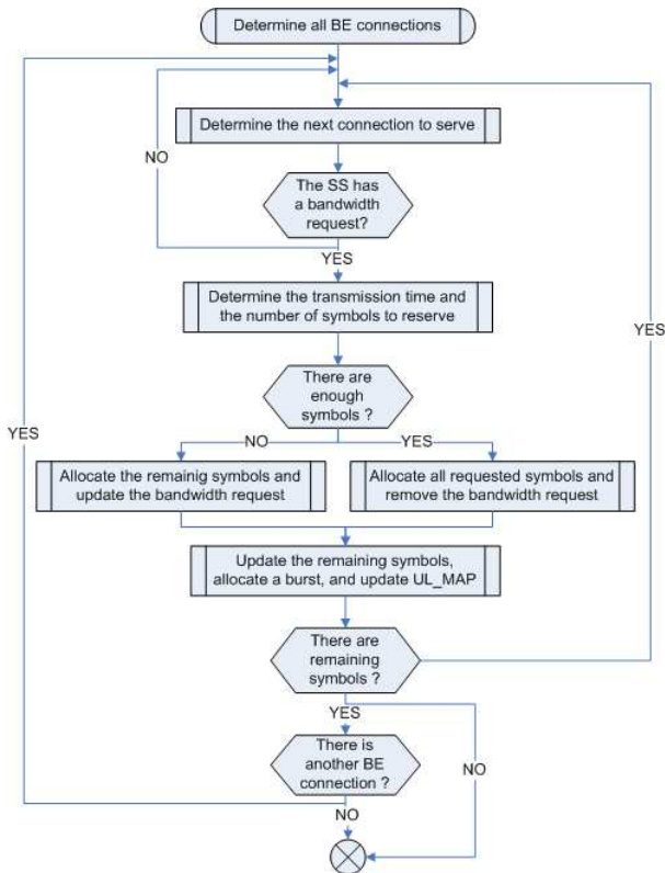
Figure 8: BE scheduling.
