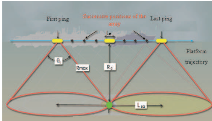
Fig. 1. SAS principle
