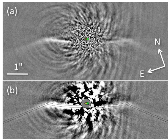
Fig. 1. High-contrast NACO H -band images of HD 61005, a) reduced with LOCI, b) reduced with ADI. The slits used for photometry are overlaid. The curved slit traces the maximum surface brightness of the lower ring arc, while the rectangular boxes enclose the streamers. In both images the scaling is linear, and 1'' corresponds to a projected separation of 34.5 AU. The arc-like structures in the background are artifacts of the observation and reduction techniques, and are asymmetric because the field rotation center was offset from the star. The region with insufficient field rotation is masked out. The plus marks the position of the star, the cross the ring center.
