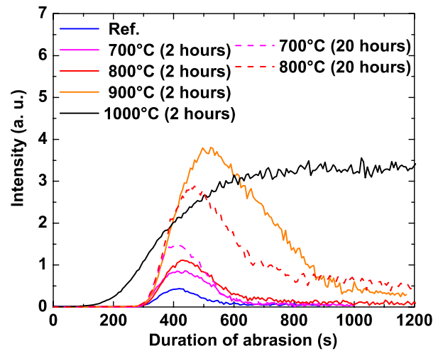
Figure 5. SIMS depth profile signal related to oxygen
