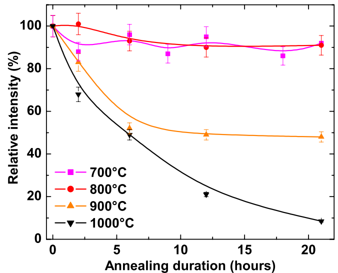
Figure 3. Intensity of the (002) XRD AlN peak as a function of the annealing duration
