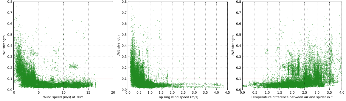
Figure 9. LWE strength \mathcal{S} as a function of the ambient wind speed (left), the top ring wind speed (middle) and the temperature difference between the spiders and the ambient air (right). The 10% red line indicates the threshold above which the LWE can be robustly stated as present during the observations.
