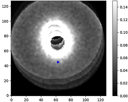
Fig. 4. Recombined K-Stacker image where the false planet candidate can be seen (indicated by the arrow). The observer noted the asymmetry of the planet spot.
