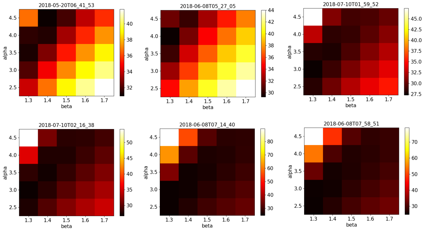
Fig. B.3: Root square error between deconvolved images and OASIS+albedo model. Each of the 6 subfigures corresponds to one of the observing epoch. Evolution of the error with respect to the \alpha and \beta parameters is then visible. Invalid pixels (missing albedo) were removed for error computation. However all pixels (inside AND outside the asteroid) are considered to take into account the residual blurring after eventual incomplete deconvolution.
