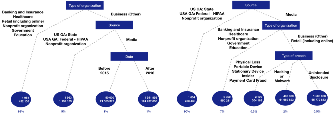
Figure 3: Trees obtained by the CART algorithm based on the quadratic (left-hand side) and the absolute (right-hand side) losses. For each leaf, the value of the empirical median (first line) and mean (second line) are given.
