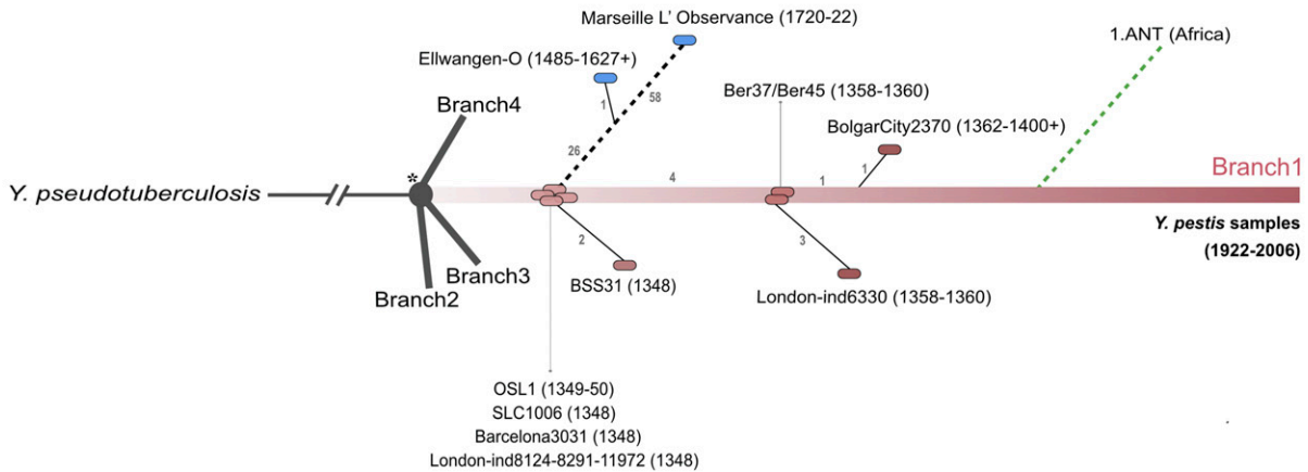
Fig. 3. Reconstruction of the phylogenetic tree and evolutionary history of Y. pestis . (A) Maximum likelihood (ML) phylogenetic tree for Y. pestis . Consisting of 126 modern Y. pestis strains and 15 ancient genomes, the tree was built using IQ-Tree (version 1.5.5) (14), which implements ModelFinder (15) to find the right substitution model before ML tree search. A total number of 2,826 polymorphic sites were used to construct the ML tree, which was visualized and edited using FigTree (version 1.2.1). Strains belonging to branch 1, branch 2, and branch 3 were collapsed for clarity. The numbers at each node indicate the bootstrap values at 1,000 replicates, SH- alrt support values at 1,000 replicates, and local bootstrap support values, respectively. The nodes indicated by black circles correspond to 100/100/100 of the support values in the same order as previously described. The asterisk marks the polytomy known as the “Big Bang.” (B) Schematic representation of the evolutionary history of Y. pestis genomes dated to the Second Plague Pandemic. Each circle represents one sample. The numbers on each branch correspond to the number of sequentially accumulated SNPs (SI Appendix).
