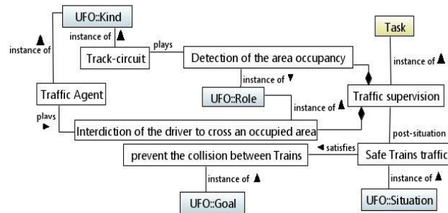
Fig. 4. The UML fragment for example illustration.
