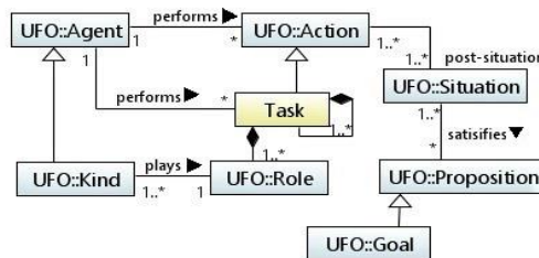
Fig. 2. UML fragment focusing on Roles and GORO concepts.
