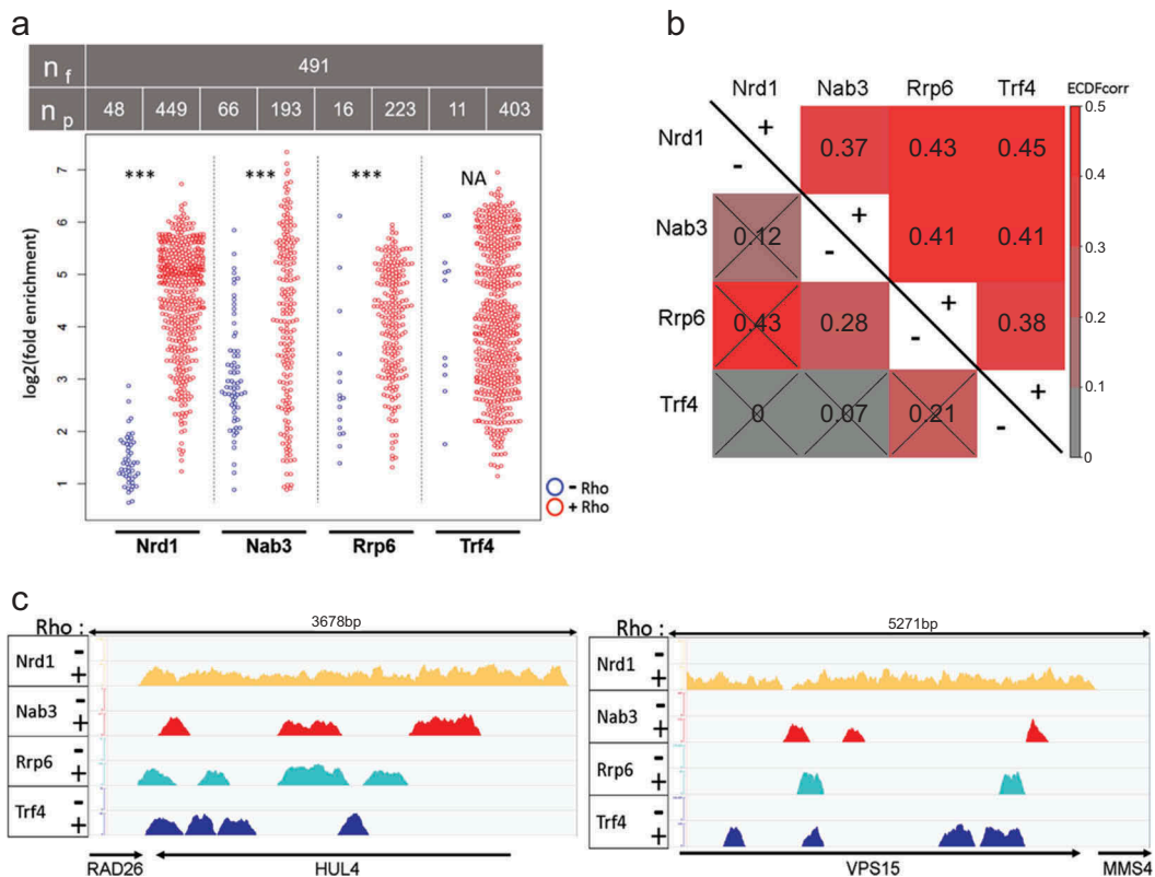
Figure 5. Rho activity mediates the stimulation of massive recruitment of QC components to Rrp6-sensitive mRNAs genomic loci. a) Beeswarm plot of \log_2 fold enrichment detected on the rescued mRNAs genomic loci obtained by ChIP-seq experiments for each indicated QC protein. The ChIP signals are shown as open dots in blue for -Rho and in red for +Rho conditions. A student t-test was used to assess the significance of enrichment differences between the -Rho and +Rho conditions with the following code 0.05>*.01>**.001>***. (NA) stands for not applicable. The table above the graphs gives the number of analysed features ( n_f ) and the number of loci possessing at least one peak for each protein ( n_p ) in -Rho or +Rho conditions. b) Correlogram of Empirical Distribution Cumulative Function correlation area (calculated with the geometricorr package) for each protein pairs over the analysed genomic loci under Rho perturbation (“+” symbols) or not (“-” symbols). The crossed boxes indicate the absence of correlation significance. c) IGV snapshots of ChIP-seq peaks mapped over two rescued mRNAs genomic loci. The ChIP signals for each protein are shown both for -Rho and +Rho conditions.
