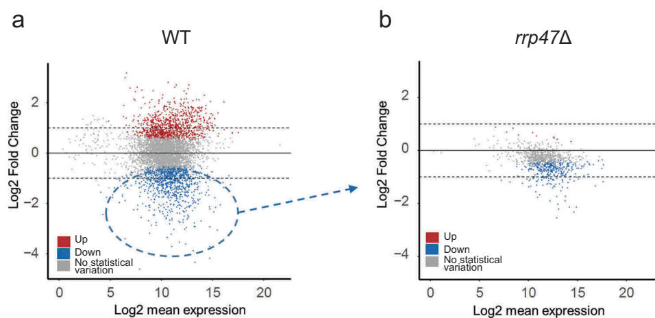
Figure 1. Fate of a subpopulation of mRNAs down-regulated by Rho action in Wt cells and their rescue in a strain with a deletion of RRP47 , i.e. depleted of Rrp6. a) MAplot of the \log_2 FoldChange ratios of the mRNAs between -Rho and + Rho conditions ( \log_2(\pm Rho) ) from WT cells distinguishes three sub-populations: statistically upregulated in red, statistically downregulated in blue and no statistical variation in grey. The dashed blue circle surrounds the population of interest which is down-regulated. b) MAplot as in a but for the mRNAs obtained from rrp47Δ cells and focuses only on the subset of mRNAs that were down-regulated in WT cells as determined in a.
